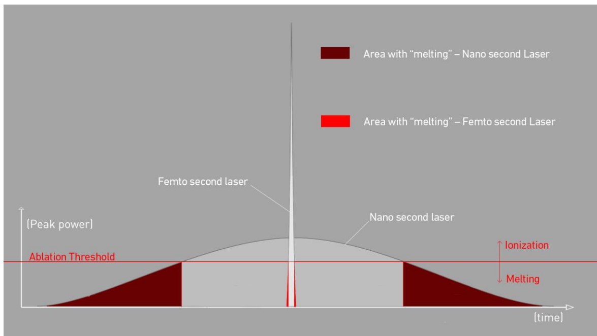
Fig. 4 showing the pulse duration and behavior of Nano versus Femto second lasers
